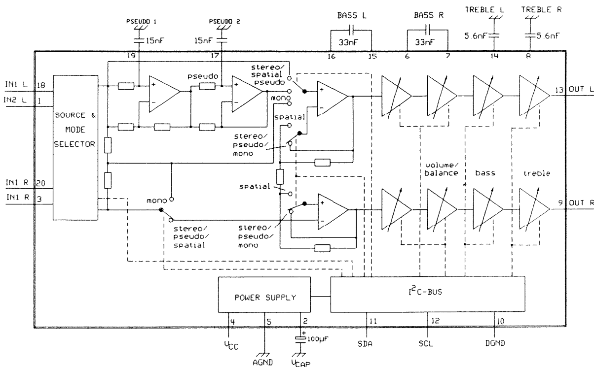
BLOCK DIAGRAM OF TDA8425
