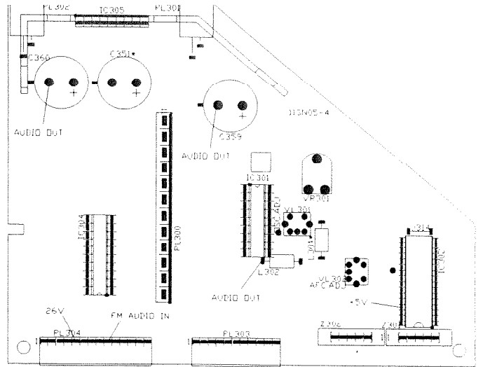
11SN05 SECAM-L NICAM STEREO MODULE
