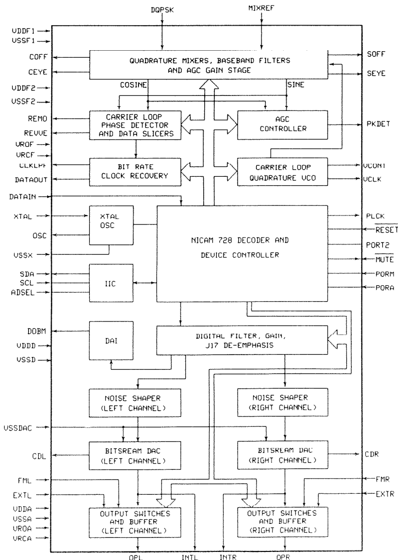
BLOCK DIAGRAM OF SAA7283
