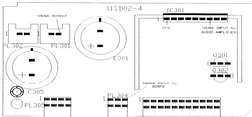
11SD02 SOUND MODULE
