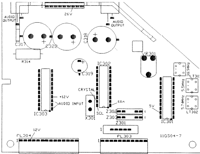
11GS04 GERMAN STEREO MODULE
